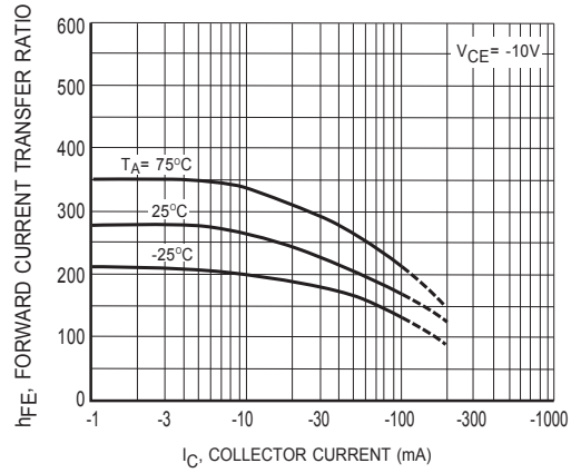
Figure7 h_{FE}-I_C
