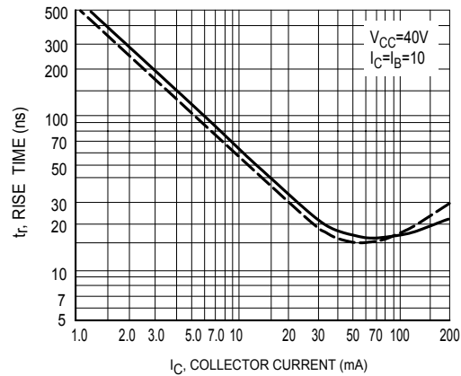
Figure 4. Rise Time
