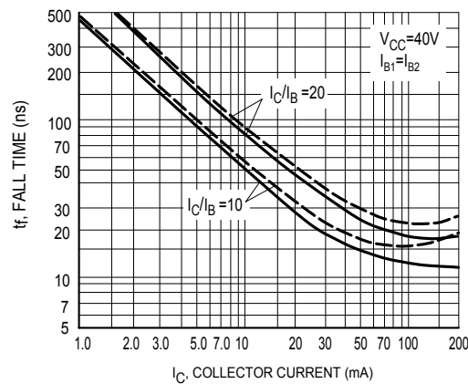
Figure 6. Fall Time
