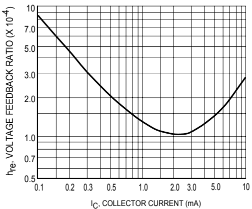
Figure 12. Voltage Feedback Ratio
