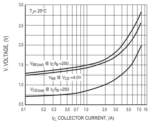
Figure7 "ON" VOLTAGES
