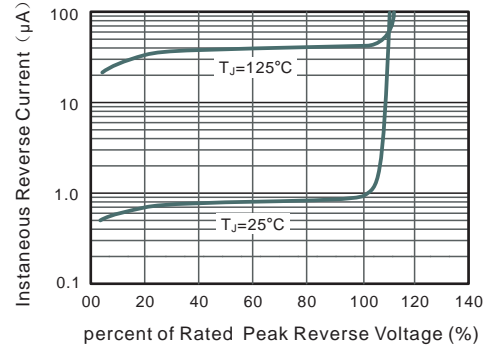
FIG.2 MAXIMUM REVERSE CHARACTERISTICS
