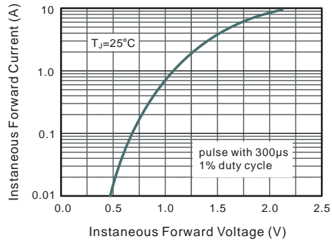
FIG.3 MAXIMUM INSTANTANEOUS FORWARD CHARACTERISTICS
