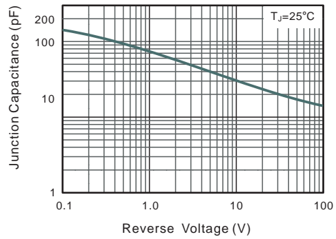
FIG.4 TYPICAL DIODE CAPACITANCE
