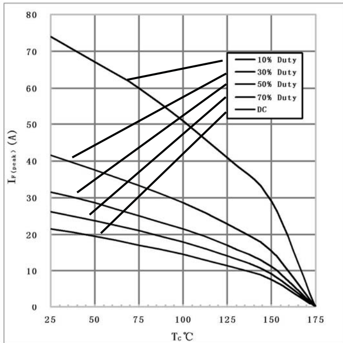
3) Current Derating
